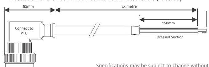
Illustration of a CA-JCMX-XX Not Pre-Terminated Cable (Dressed)
