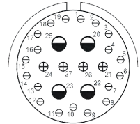
Connector (Pre-Terminated)
