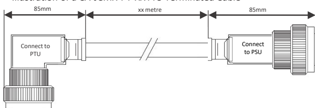
Illustration of a CA-JCMX-PT-XX Pre-Terminated Cable
