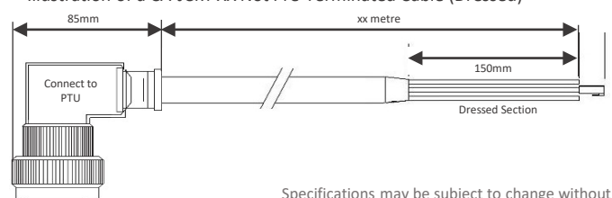
Illustration of a CA-JCM-XX Not Pre-Terminated Cable (Dressed)
