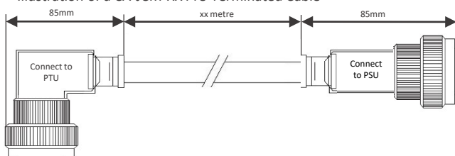
Illustration of a CA-JCM-XX Pre-Terminated Cable
